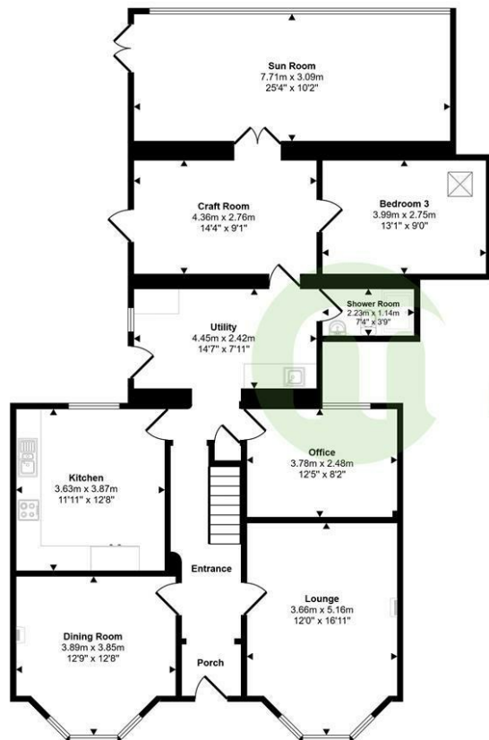
Ground Floor Approx 137 sq m / 1479 sq ft
